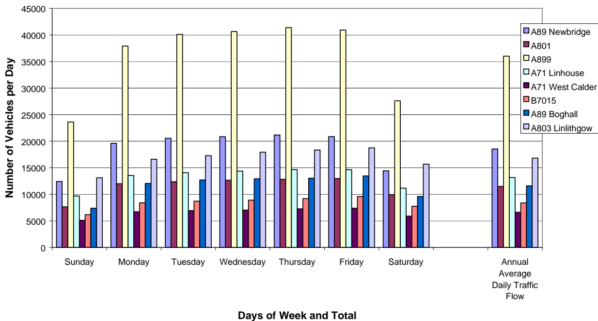
Annual Average 24 Hour Daily Figures and Annual Average Daily Traffic Flow 01/01/99 to 31/12/99
